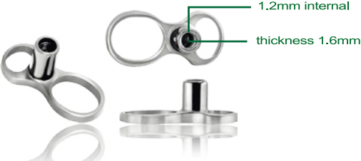
TDAO TIT. OPEN STYLE DERMAL ANCHOR GAUGES ① HEIGHT ② 1.6mm (1.2mm internal) 1.5,2.0,2.5mm
